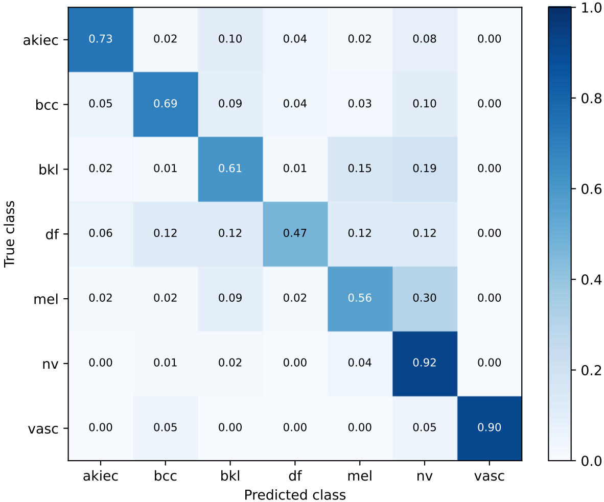
efficientnet_b0 | final locked test Row-normalized confusion matrix
