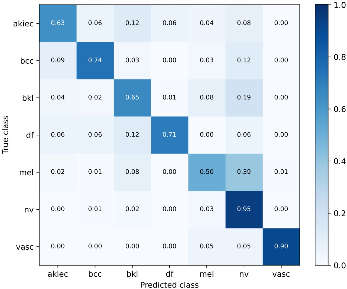
efficientnet_v2_s | final locked test Row-normalized confusion matrix
