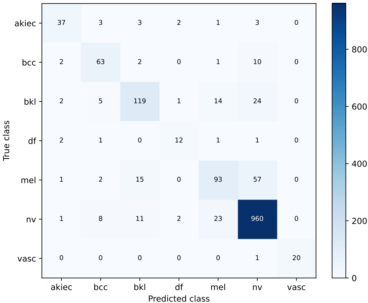
S31 equal ensemble | final locked test Confusion matrix
