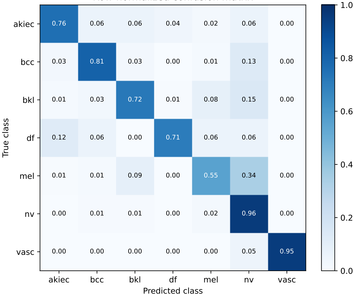
S31 equal ensemble | final locked test Row-normalized confusion matrix
