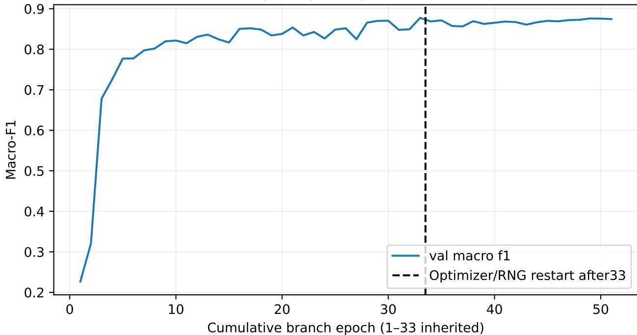
S97 ancestral trajectory + separate warm-start branch
