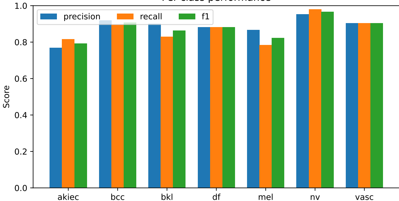
S97 warm-start | exploratory validation | best_accuracy Per-class performance
