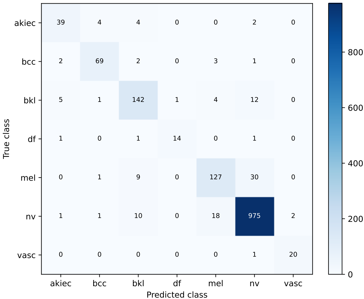
S97 final branch checkpoint | exploratory validation Confusion matrix
