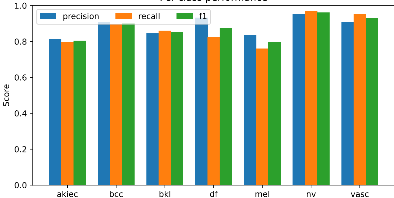
S97 final branch checkpoint | exploratory validation Per-class performance
