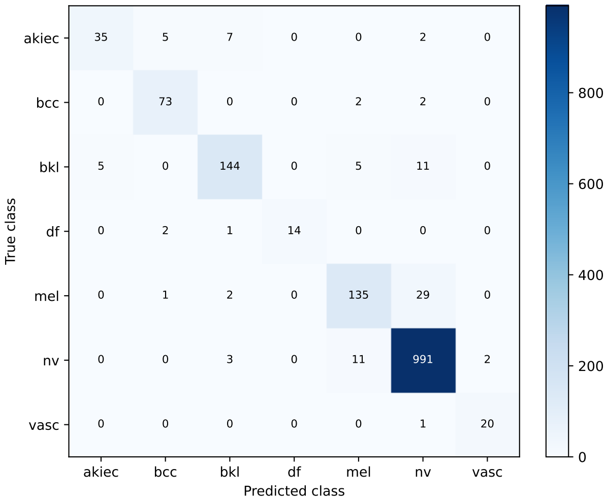
S98 fixed inherited CBAM replacement | exploratory validation Confusion matrix
