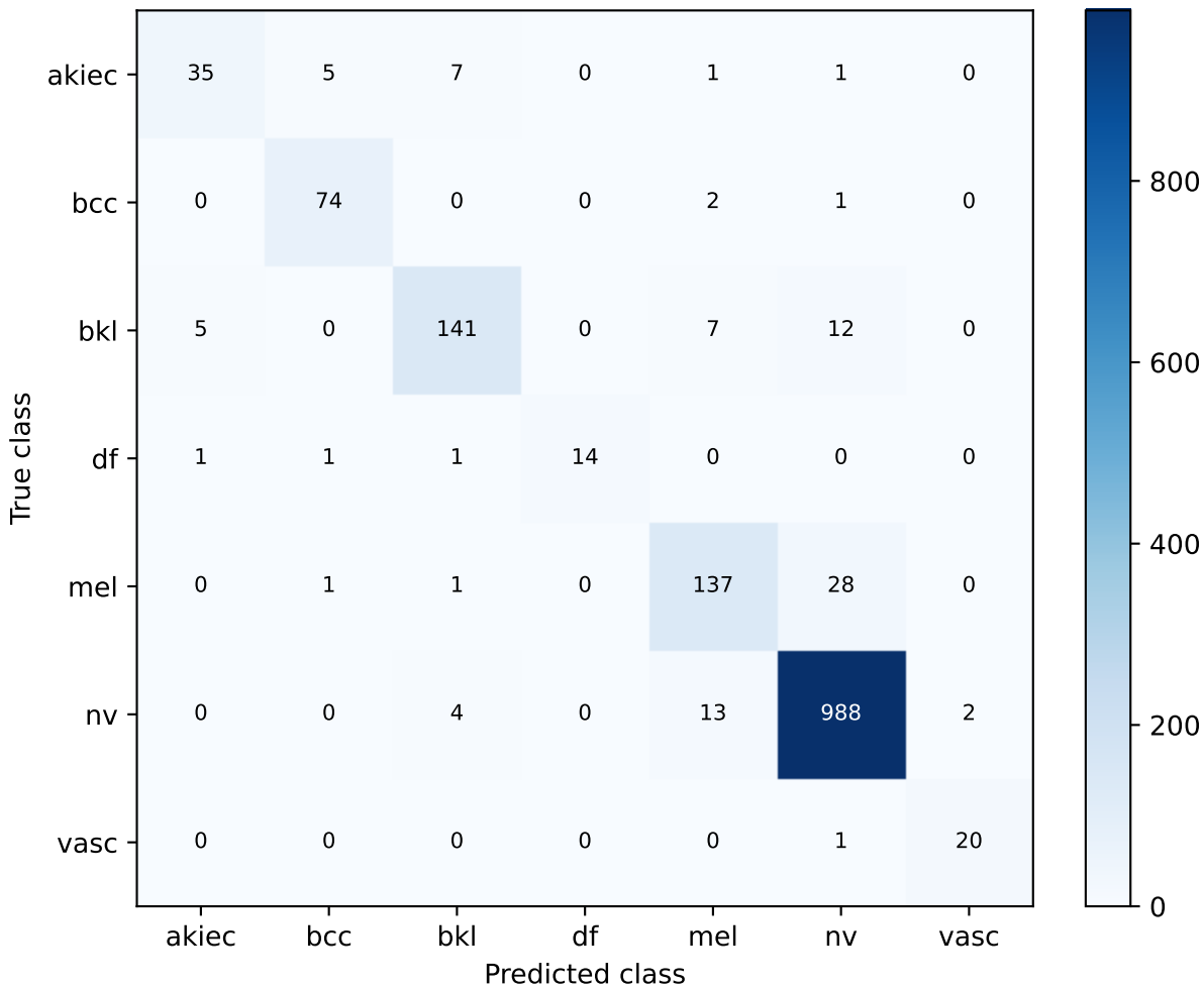
S86 saved-member addition | exploratory validation Confusion matrix
