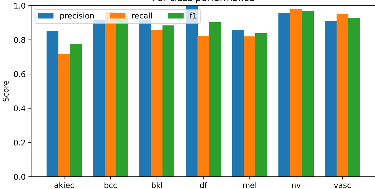
S86 saved-member addition | exploratory validation Per-class performance
