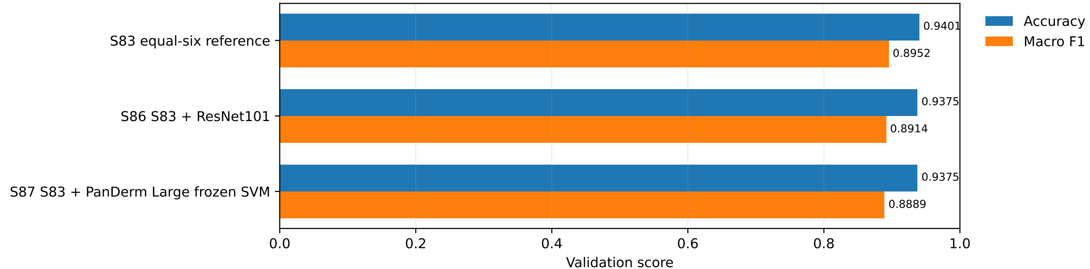
Bounded saved-model expansion | exploratory validation
