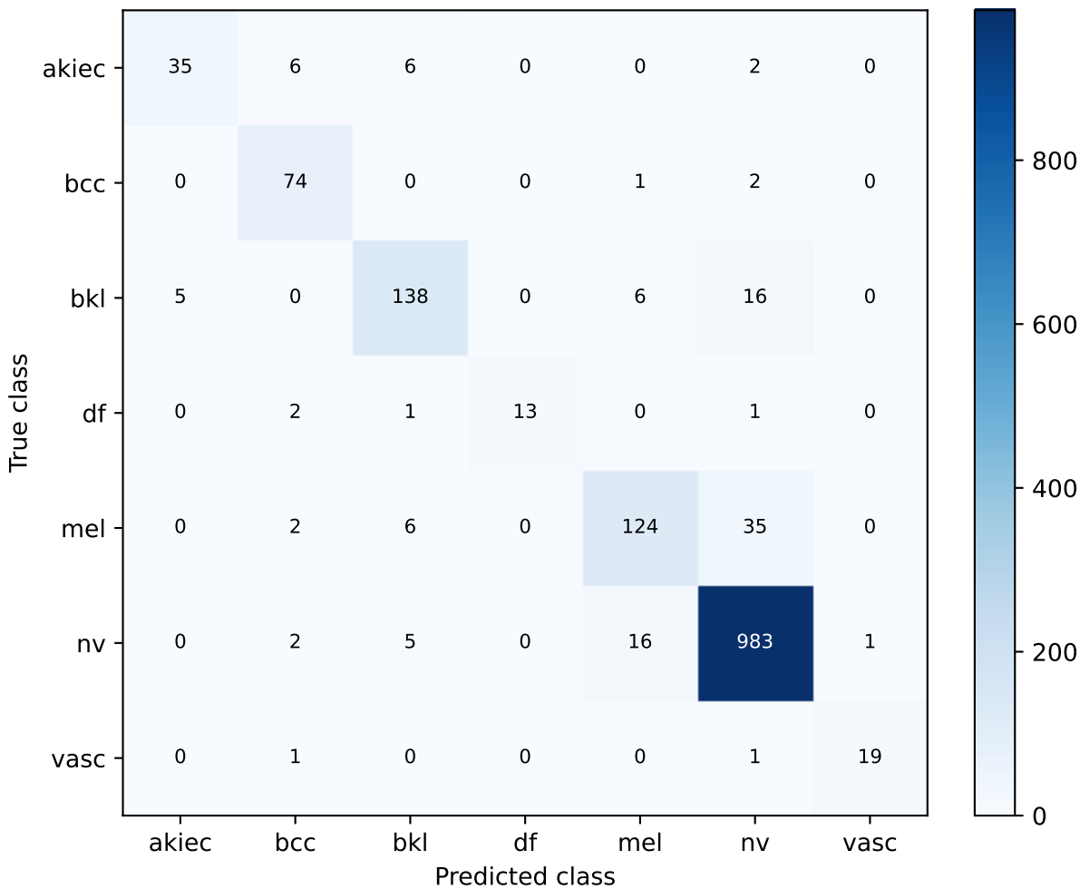
S51 current four-model four_view_tta | exploratory validation Confusion matrix
