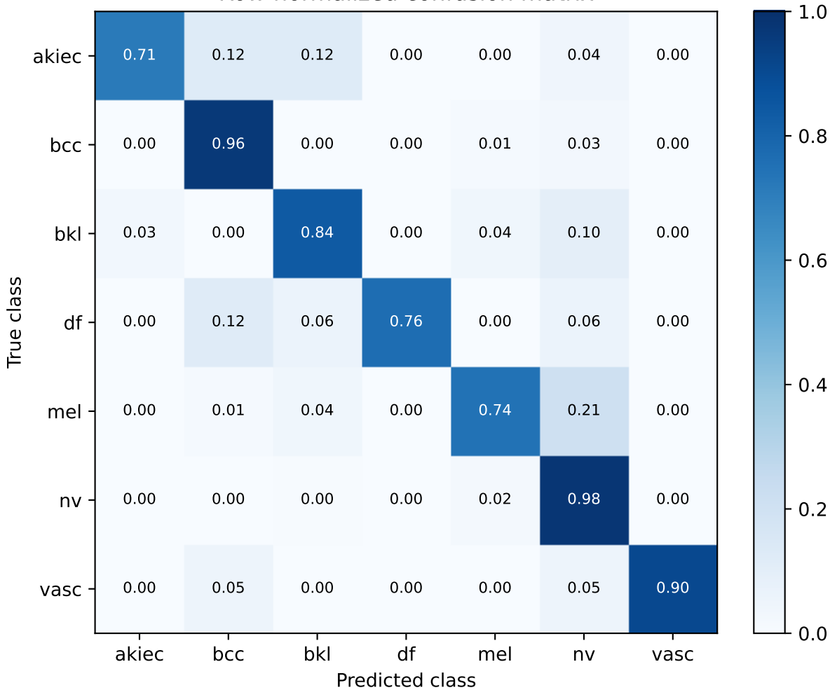
S51 current four-model four_view_tta | exploratory validation Row-normalized confusion matrix
