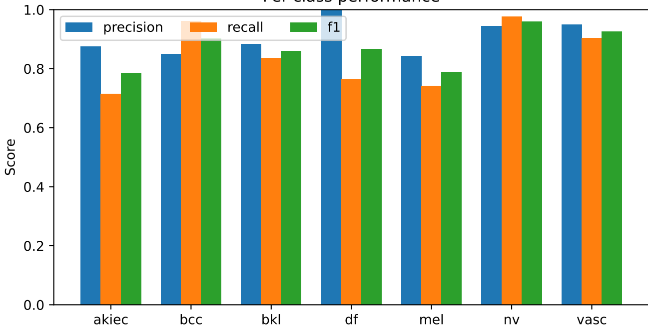
S51 current four-model four_view_tta | exploratory validation Per-class performance
