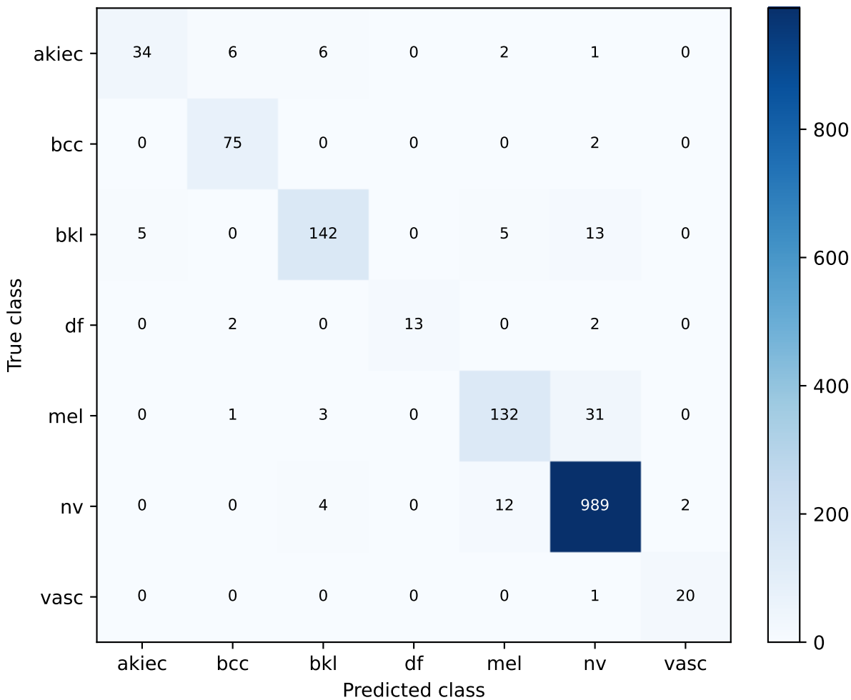
S50 current four-model identity_fp32 | exploratory validation Confusion matrix
