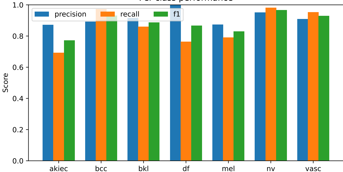
S50 current four-model identity_fp32 | exploratory validation Per-class performance
