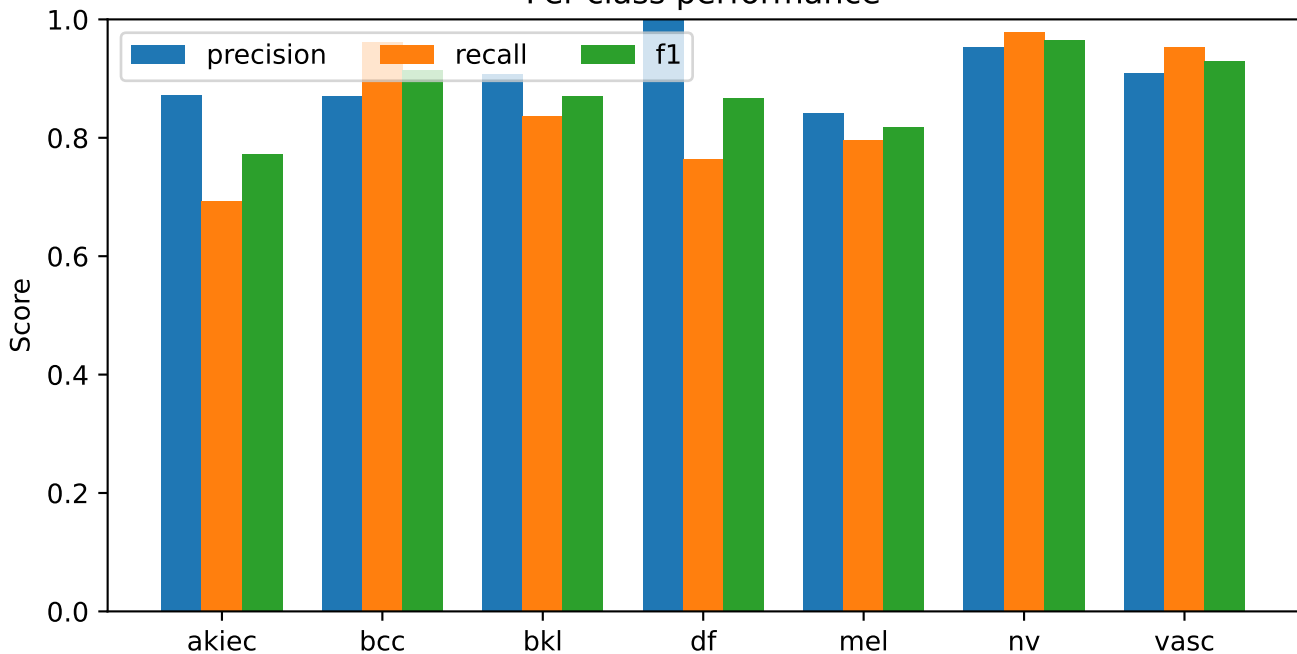
S52 fixed disagreement-only ResNet rescue | exploratory validation Per-class performance
