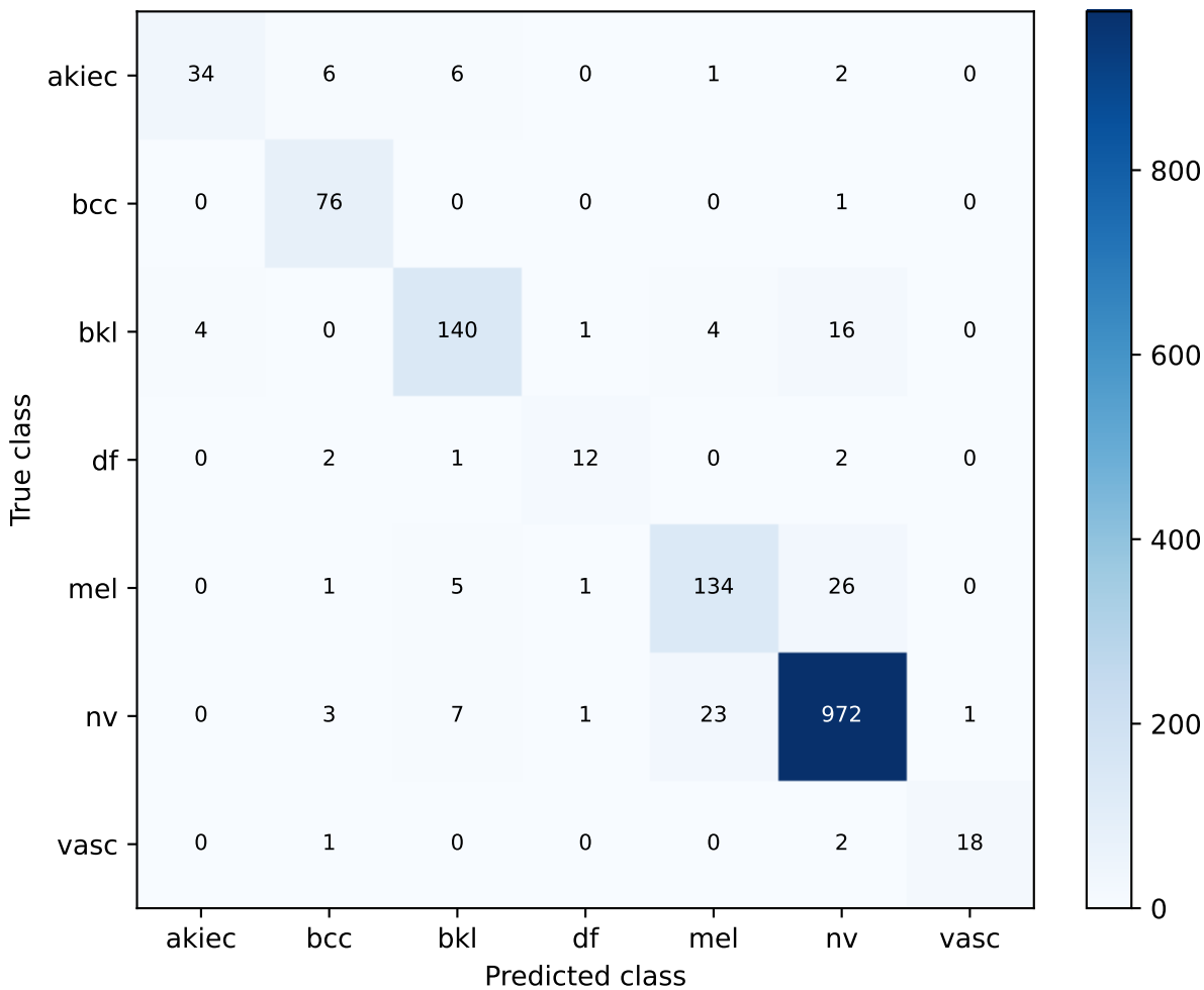
convnext_small | exploratory_image_level validation Confusion matrix
