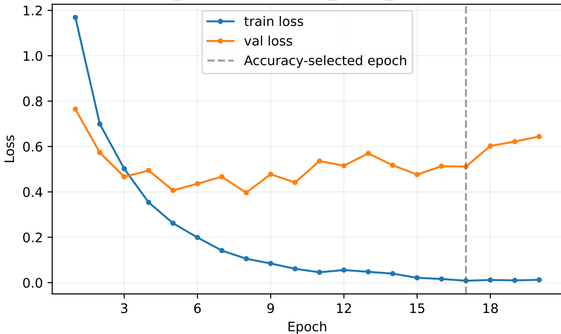
convnext_small | exploratory_image_level validation
