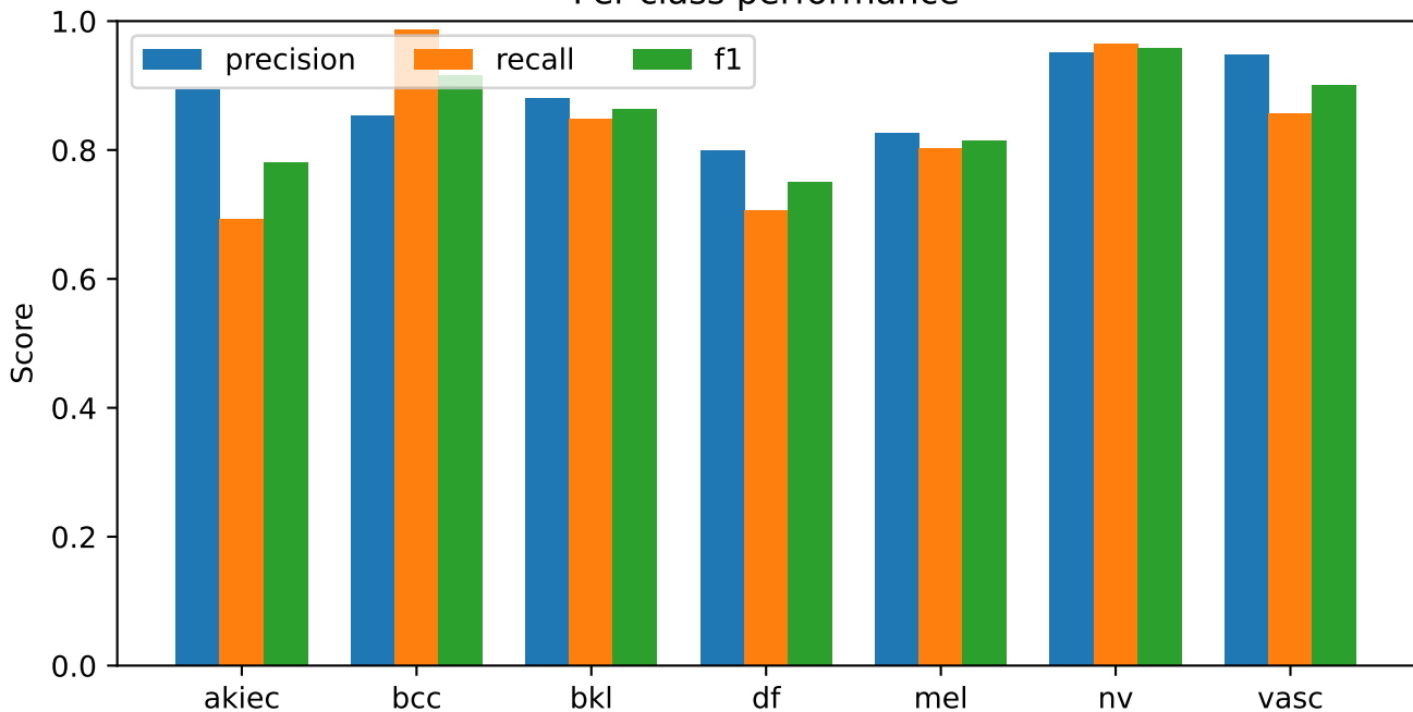
convnext_small | exploratory_image_level validation Per-class performance
