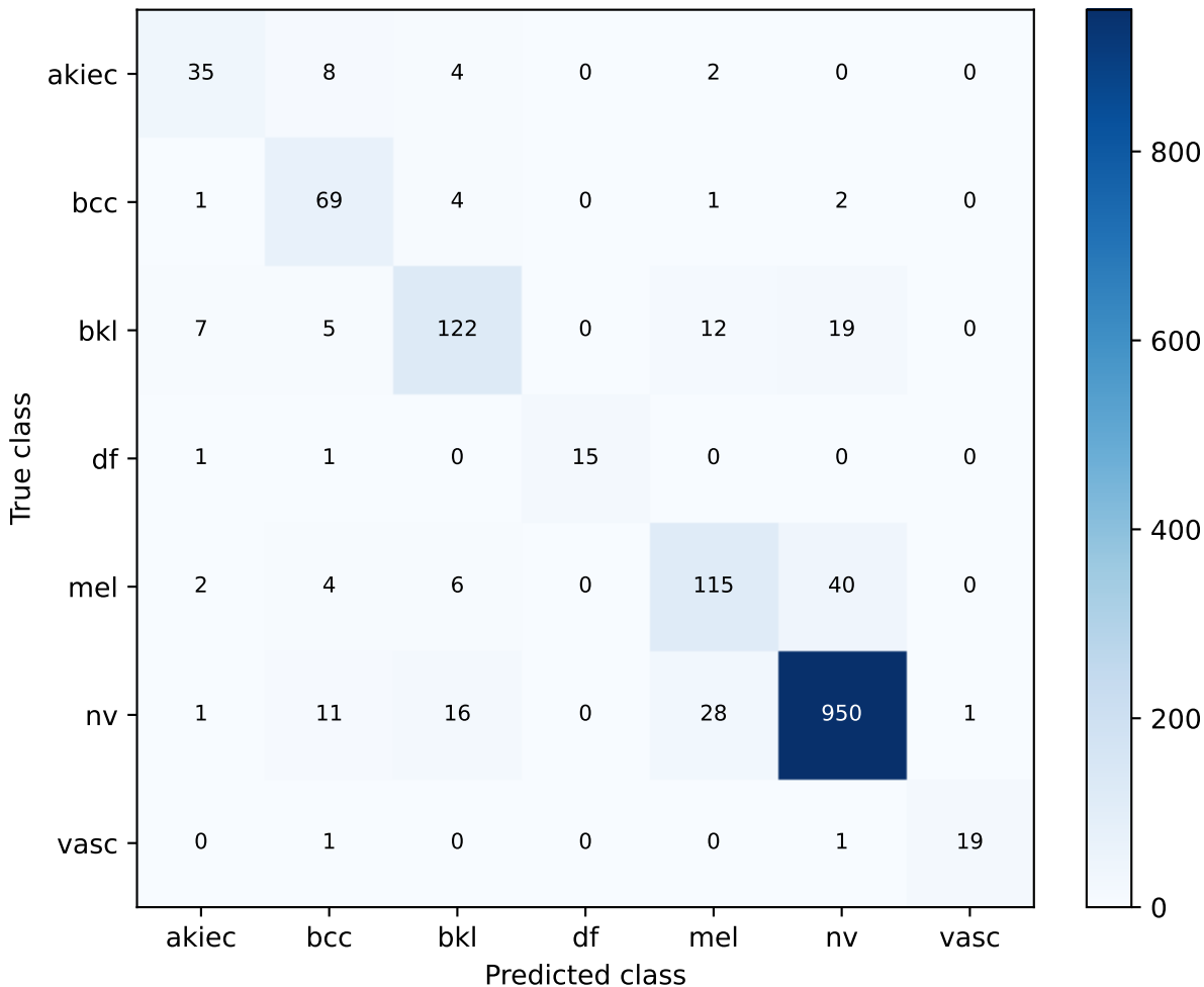
Four B0 resolution streams Historical exploratory_image_level validation Confusion matrix
