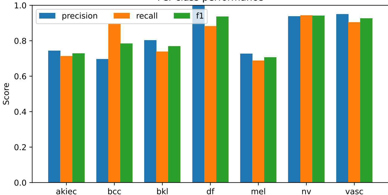
Four B0 resolution streams Historical exploratory_image_level validation Per-class performance
