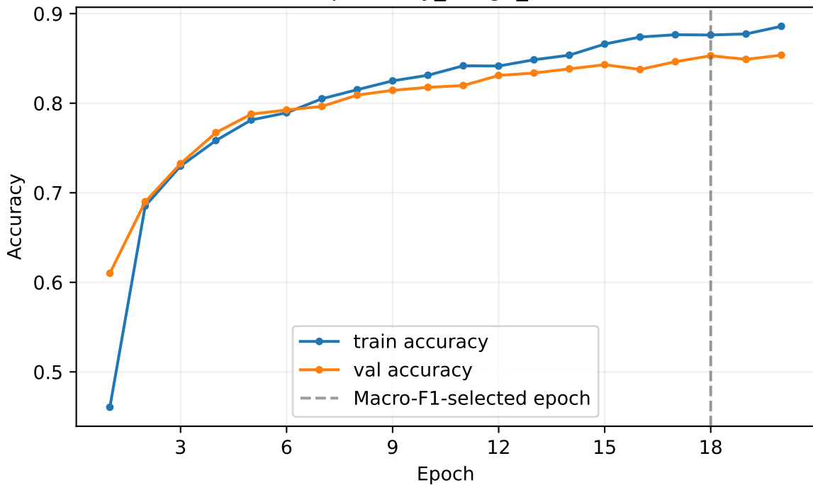
Image-level stronger augmentation Historical exploratory_image_level validation
