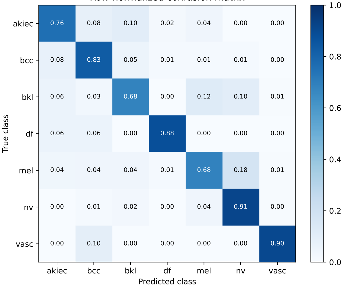
Image-level stronger augmentation Historical exploratory_image_level validation Row-normalized confusion matrix
