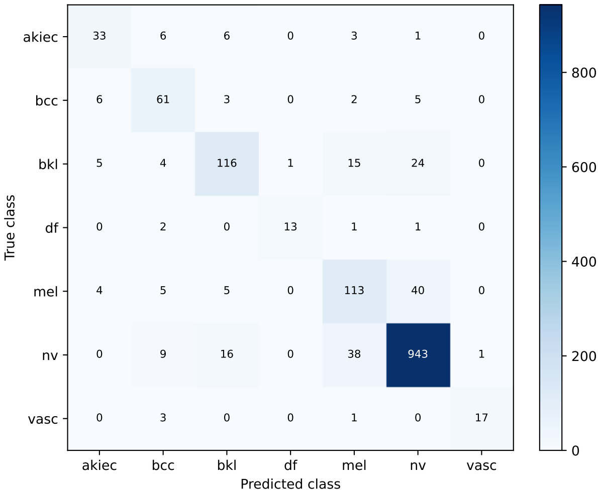
Image-level weighted B0 Historical exploratory_image_level validation Confusion matrix
