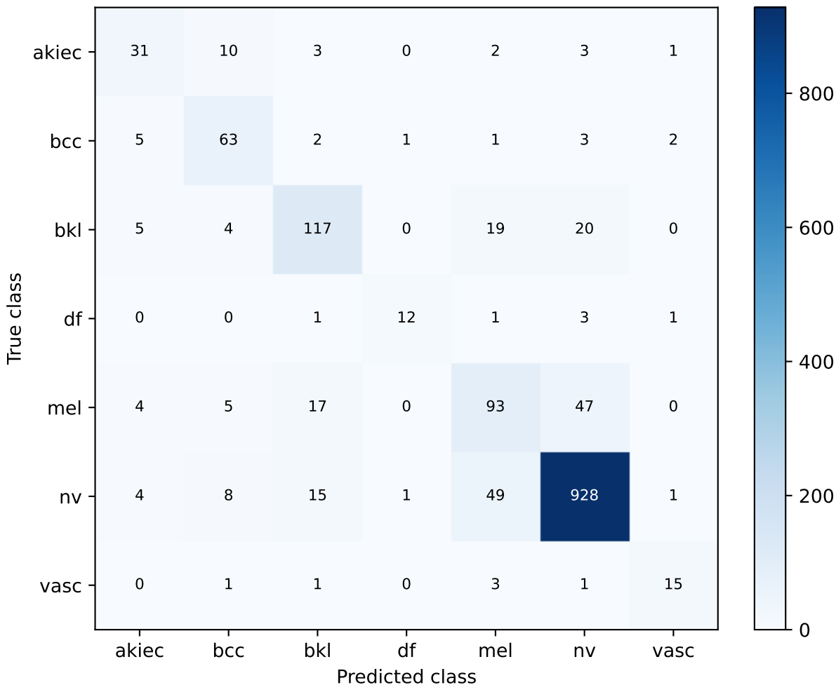
Focal B0 + CBAM Historical strict_lesion_disjoint validation Confusion matrix
