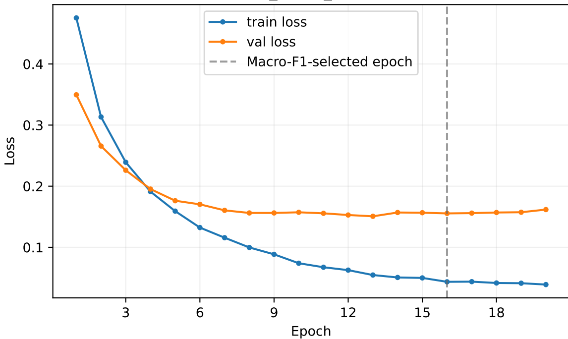
Focal B0 + CBAM Historical strict_lesion_disjoint validation
