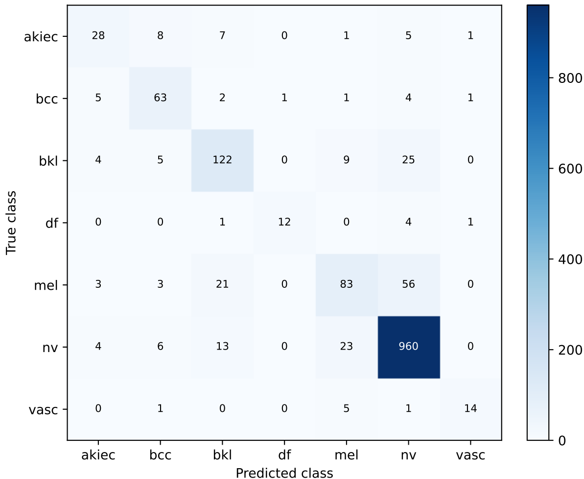
Oversampled B0 + CBAM Historical strict_lesion_disjoint validation Confusion matrix
