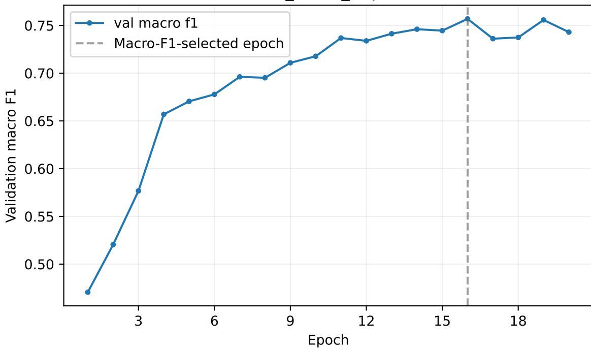
Weighted B0 + CBAM Historical strict_lesion_disjoint validation
