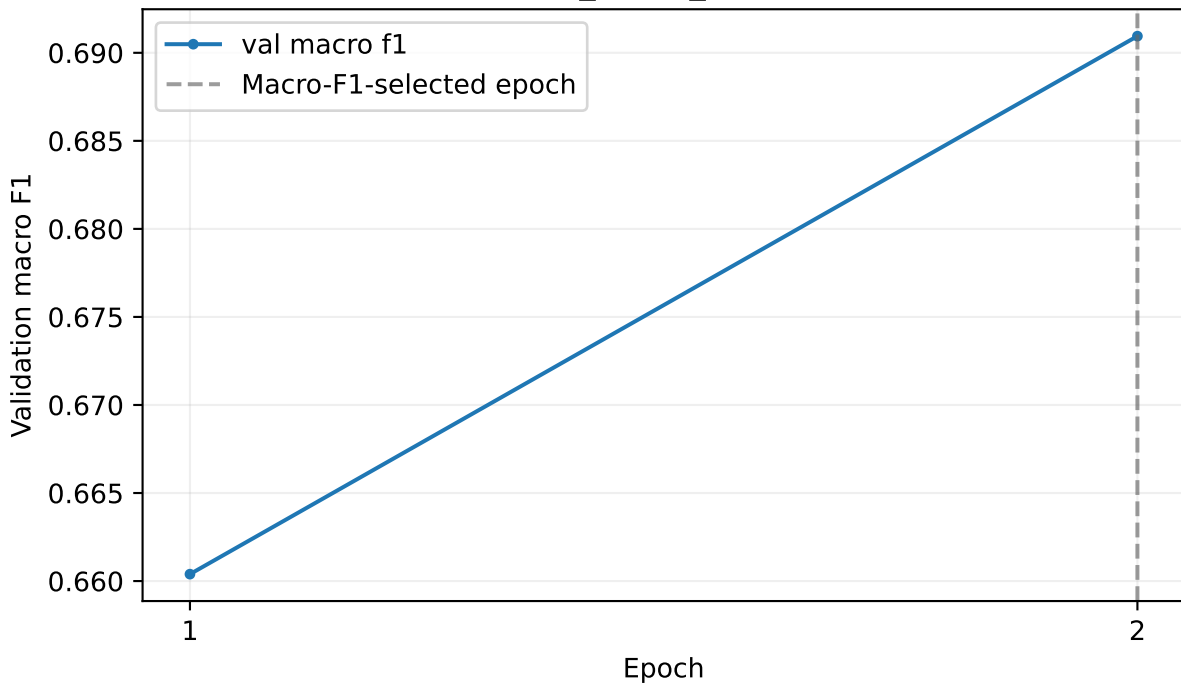
PanDerm two-epoch pilot Historical strict_lesion_disjoint validation
