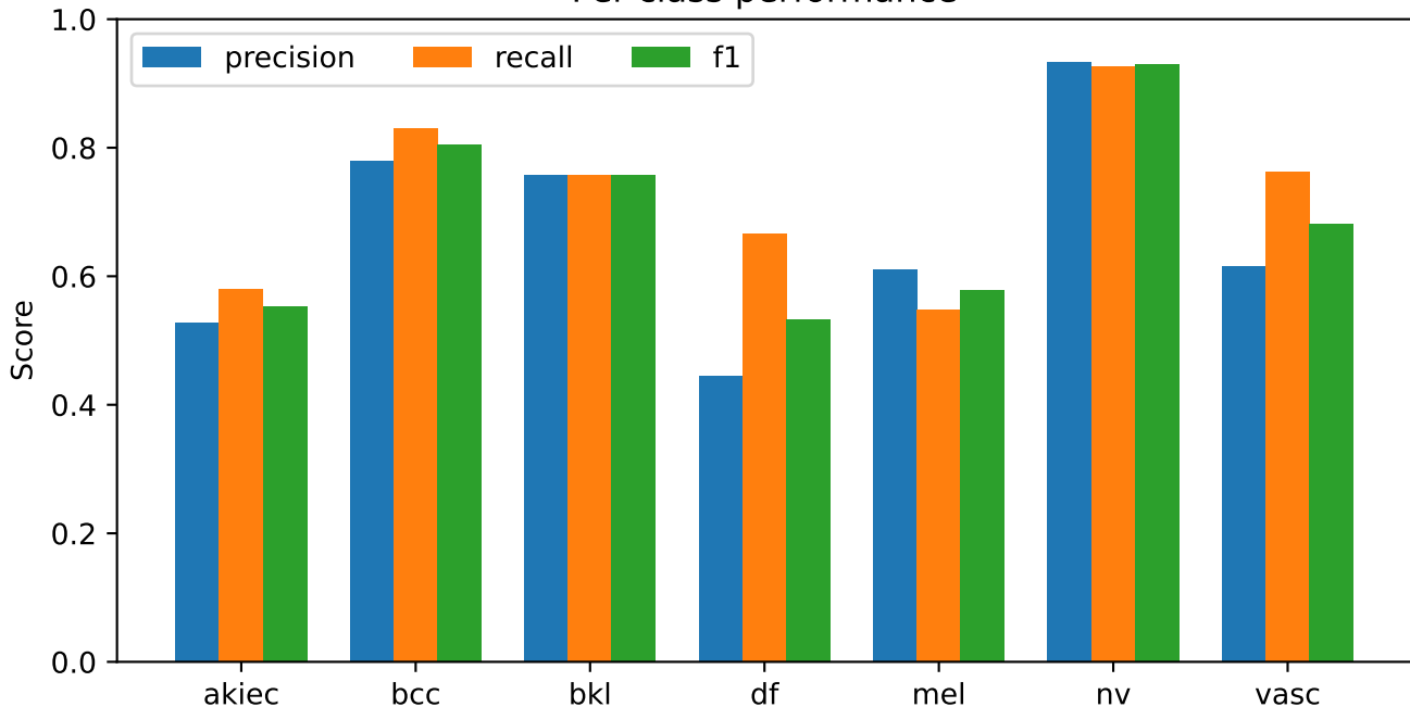
PanDerm two-epoch pilot Historical strict_lesion_disjoint validation Per-class performance
