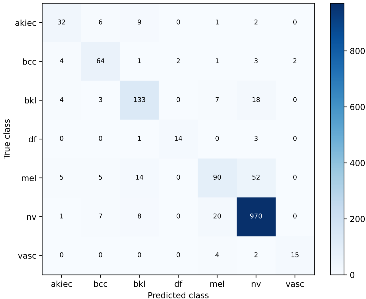
PanDerm/B0 accuracy leader Historical strict_lesion_disjoint validation Confusion matrix
