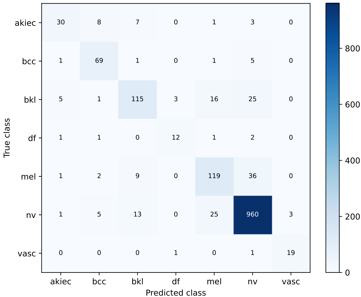
resnet101 | exploratory_image_level validation Confusion matrix
