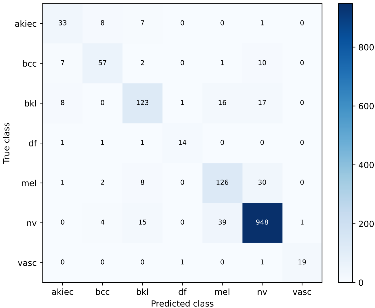
s19_resnet101_none_exploratory_seed42 | macro-F1 winner Confusion matrix
