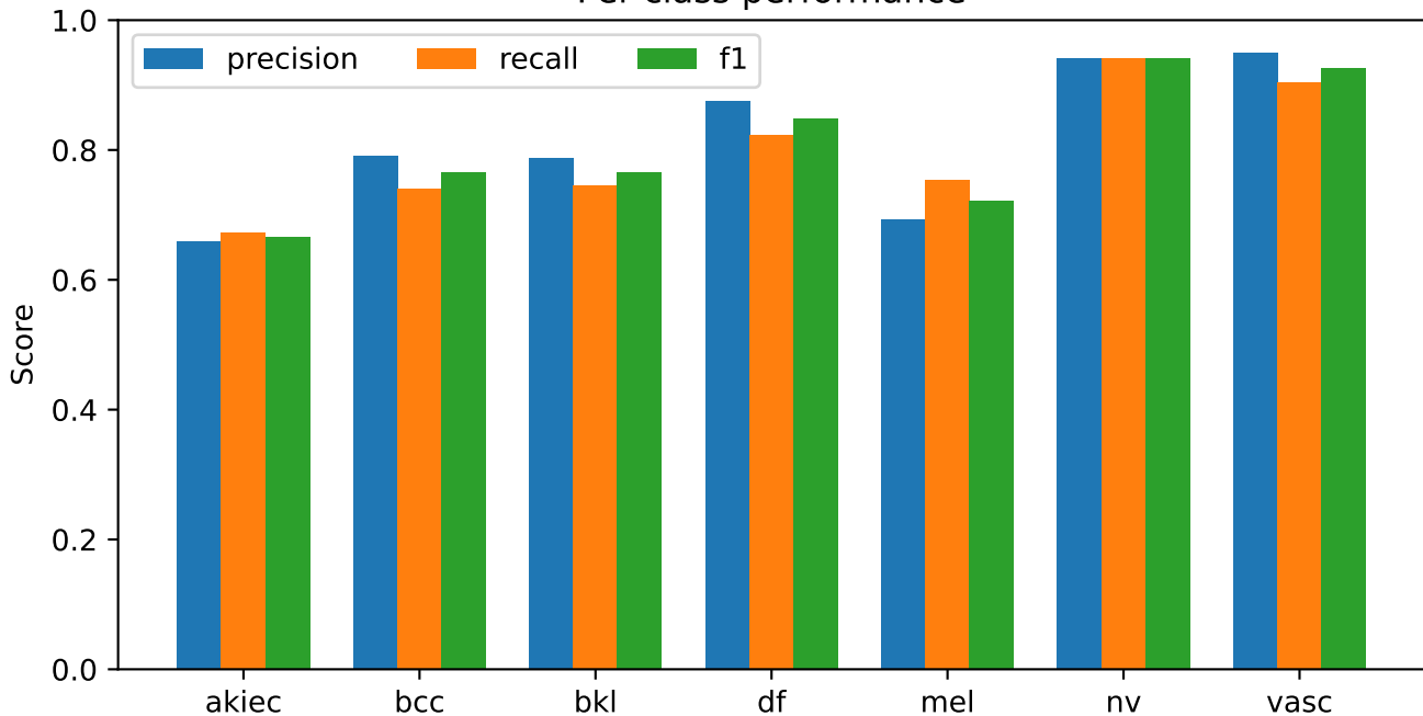
s19_resnet101_none_exploratory_seed42 | macro-F1 winner Per-class performance
