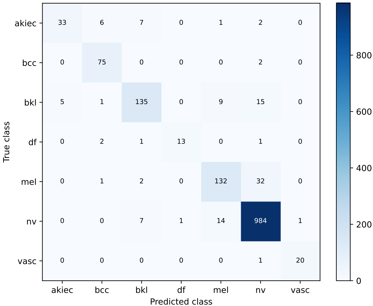
s20_final_equal_01_exploratory_seed42 | fixed soft voting Confusion matrix
