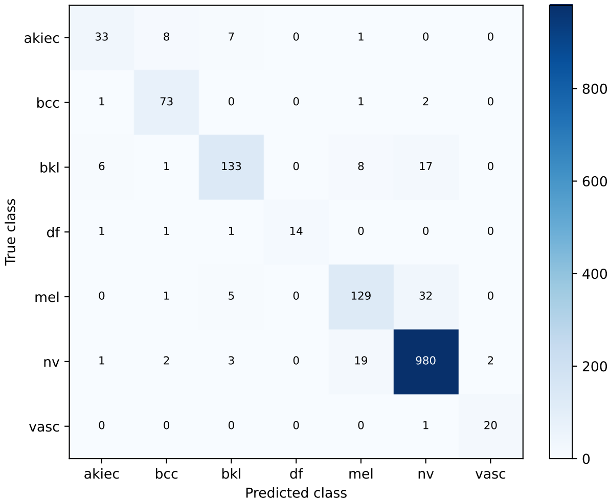
s21_final_equal_02_exploratory_seed42 | fixed soft voting Confusion matrix
