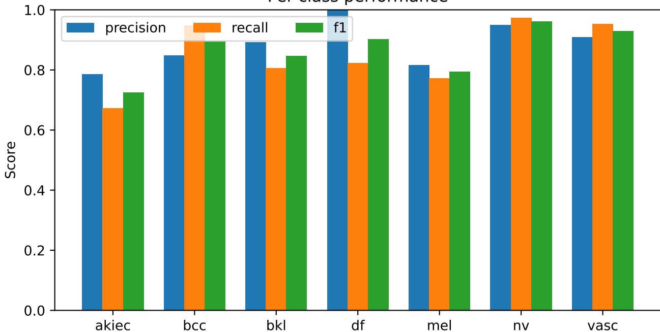
s21_final_equal_02_exploratory_seed42 | fixed soft voting Per-class performance
