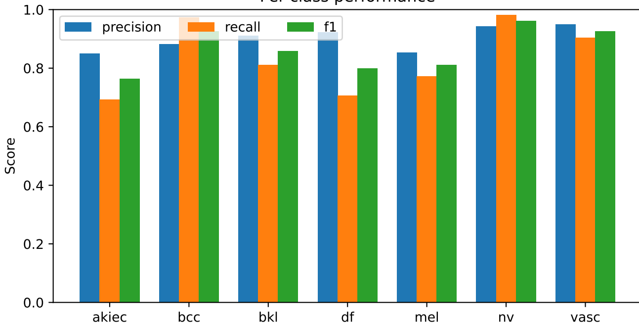
s23_final_equal_04_exploratory_seed42 | fixed soft voting Per-class performance
