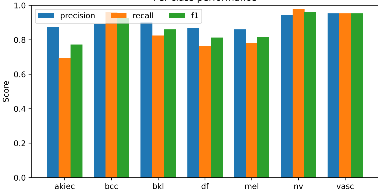
s26_final_weighted_01_exploratory_seed42 | fixed soft voting Per-class performance
