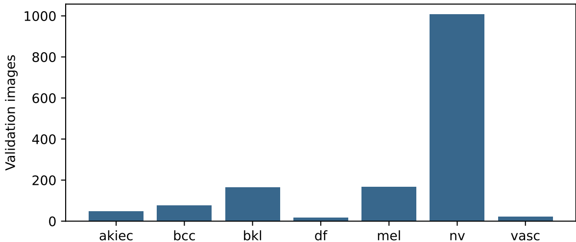
s27_final_weighted_02_exploratory_seed42 | fixed soft voting Class support
