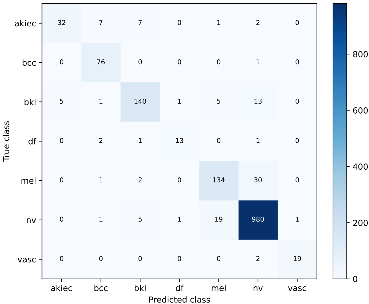
s27_final_weighted_02_exploratory_seed42 | fixed soft voting Confusion matrix
