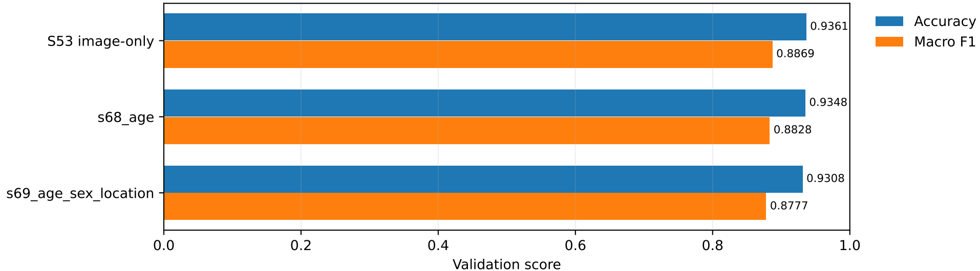
Fixed train-only metadata adjustment of retained ensemble
