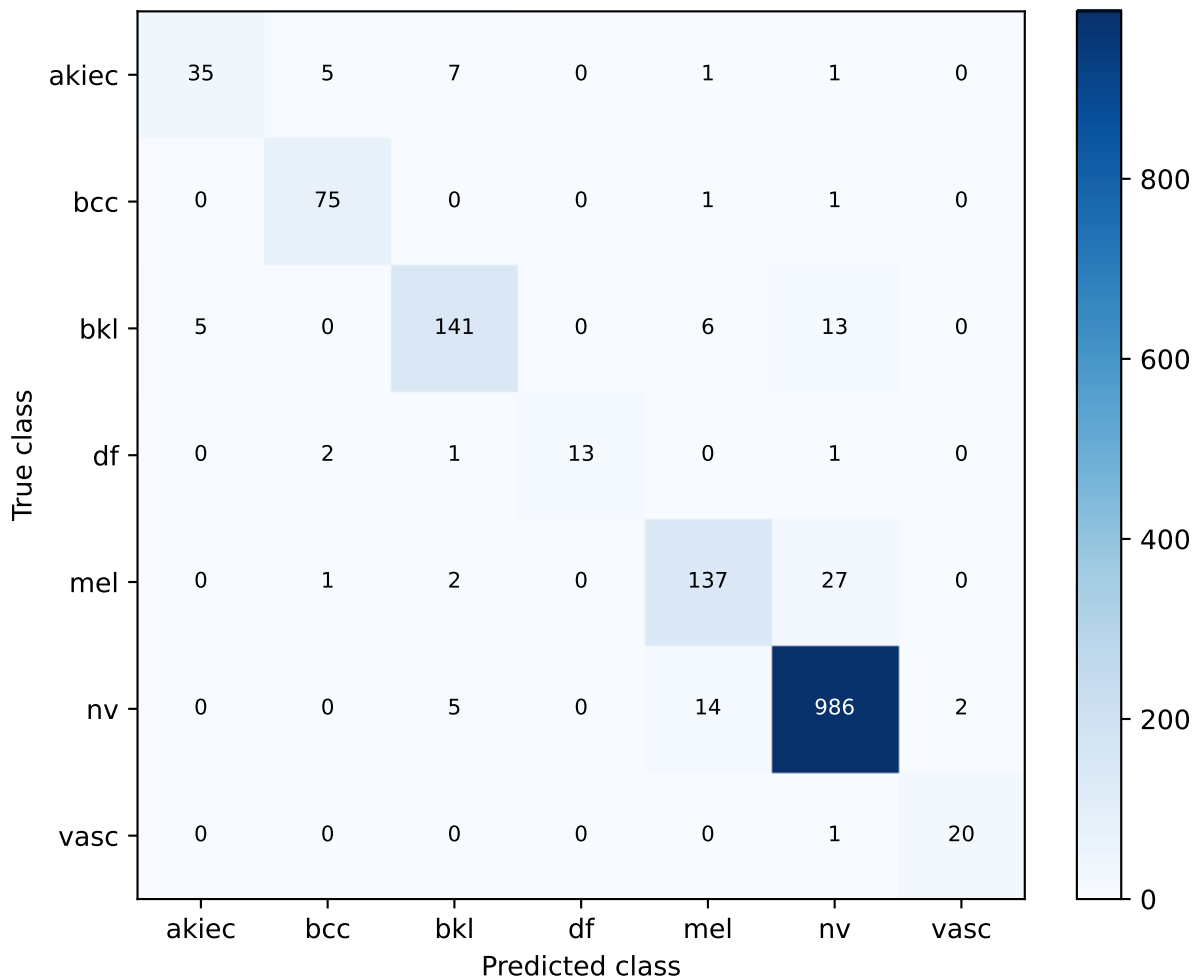
S53 retained ensemble | matched metadata reference Confusion matrix
