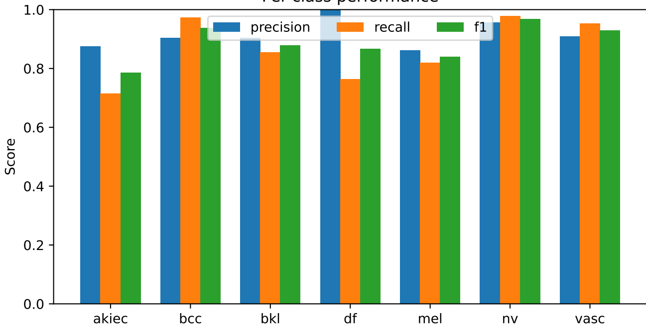
S53 retained ensemble | matched metadata reference Per-class performance
