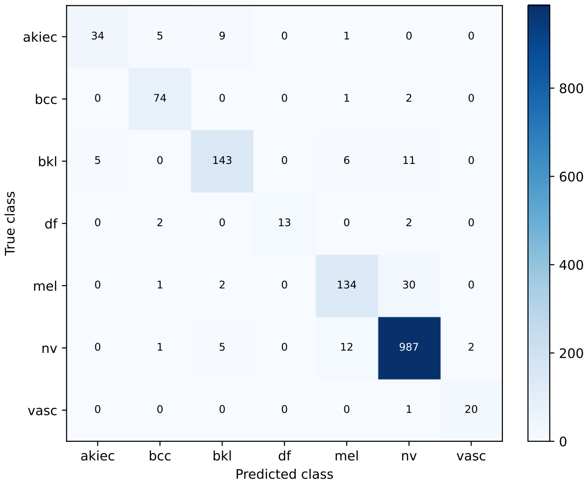
S68_AGE train-only metadata | exploratory validation Confusion matrix
