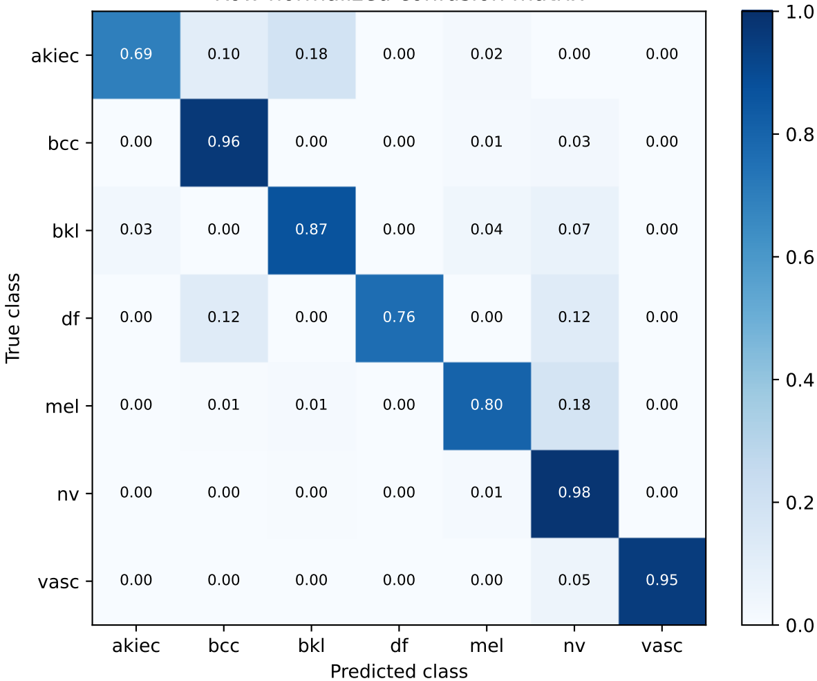
S68_AGE train-only metadata | exploratory validation Row-normalized confusion matrix
