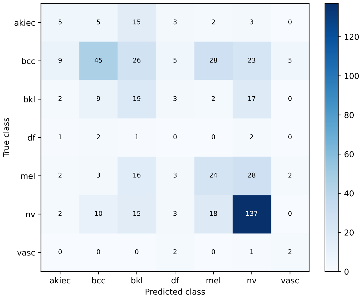
S66 ham_only | external preflight domain check Confusion matrix
