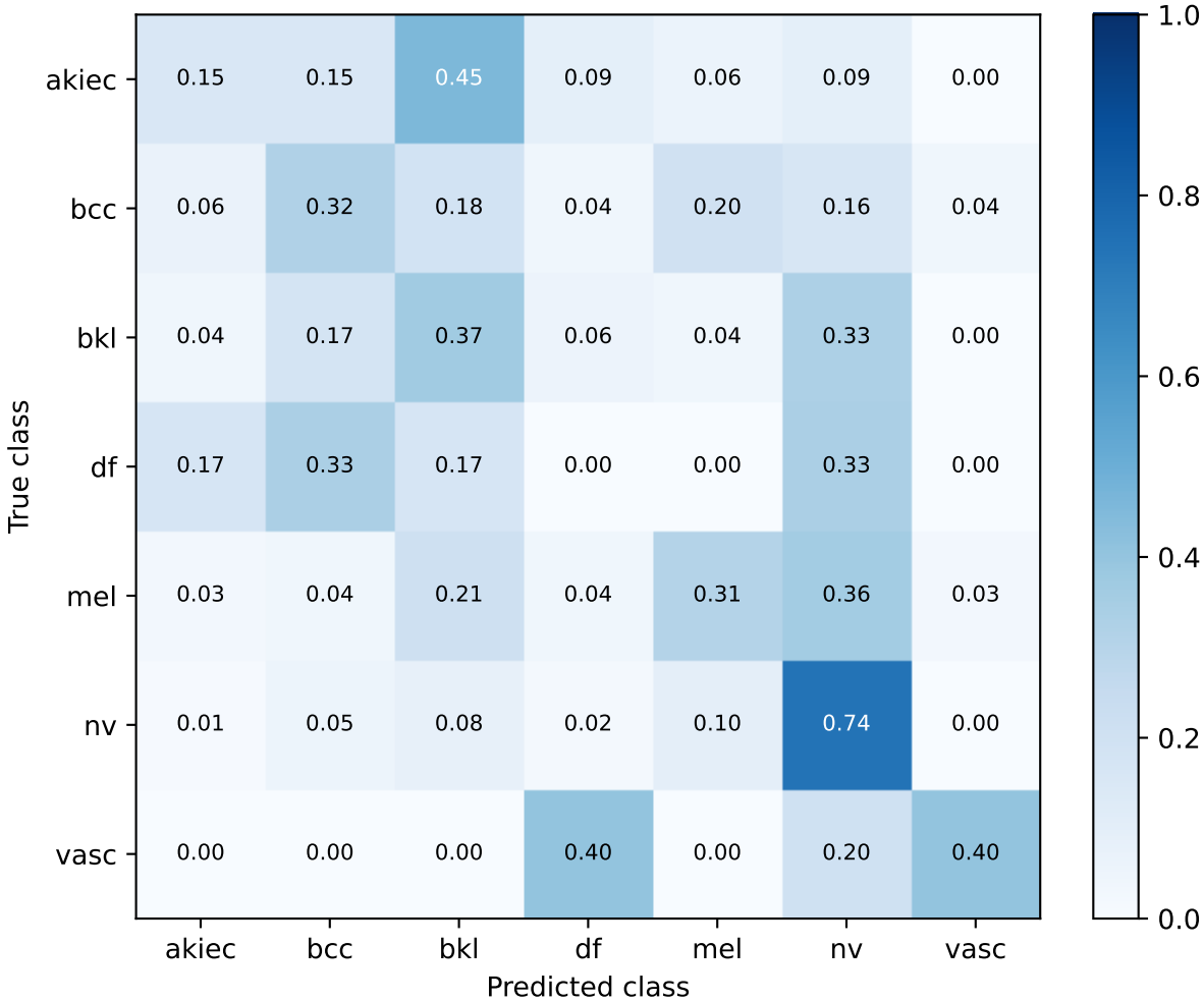
S66 ham_only | external preflight domain check Row-normalized confusion matrix
